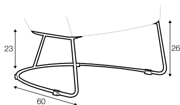
metal frame
